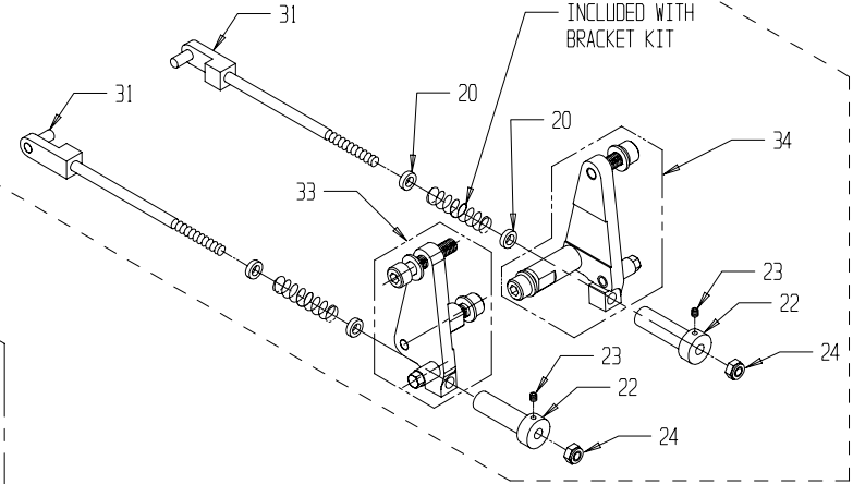
DDS KIT - ALL HEADS EXCEPT 1st : P/N 098232
