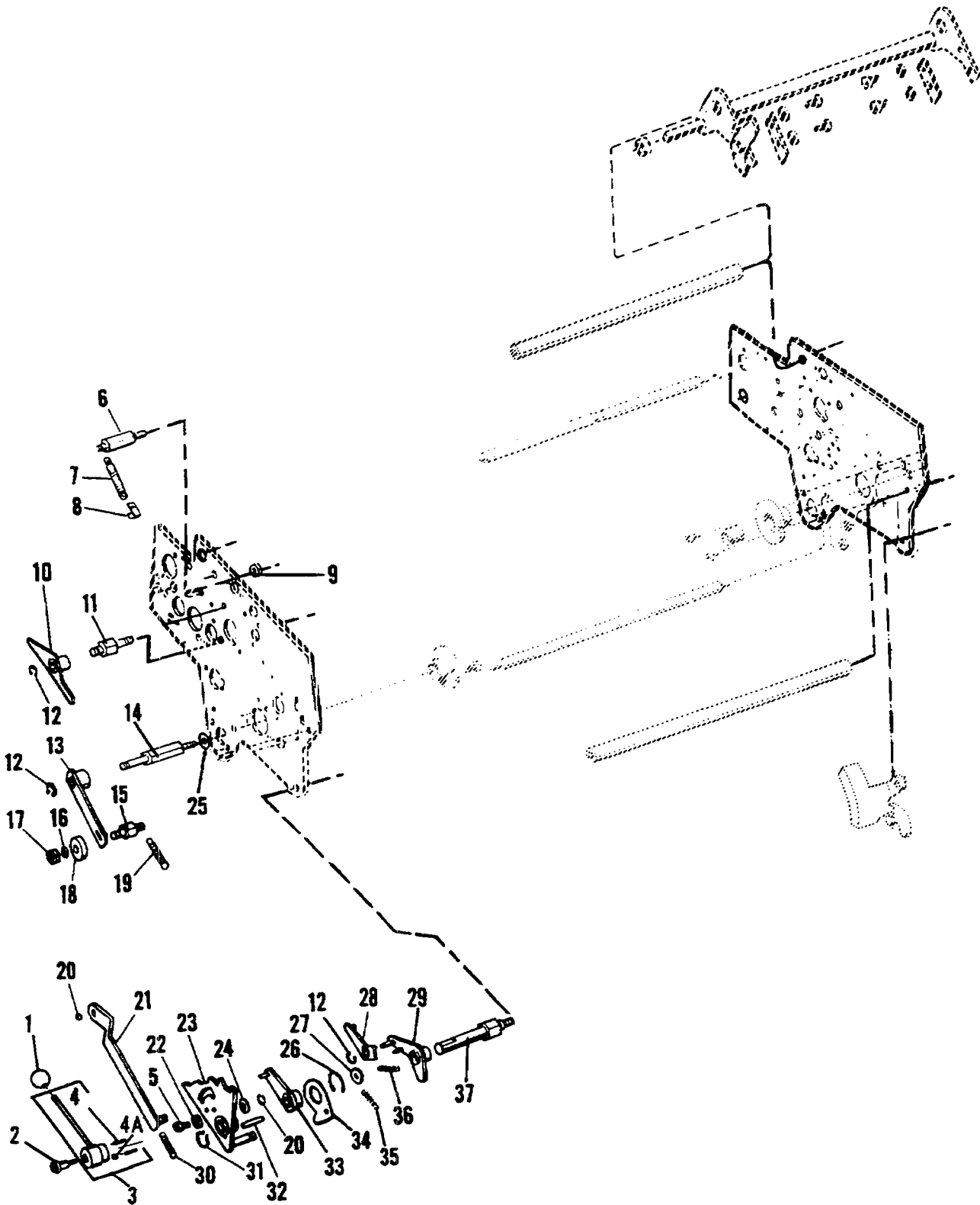
FIGURE 24A MODEL 9805/9810 Operation Control Lever
